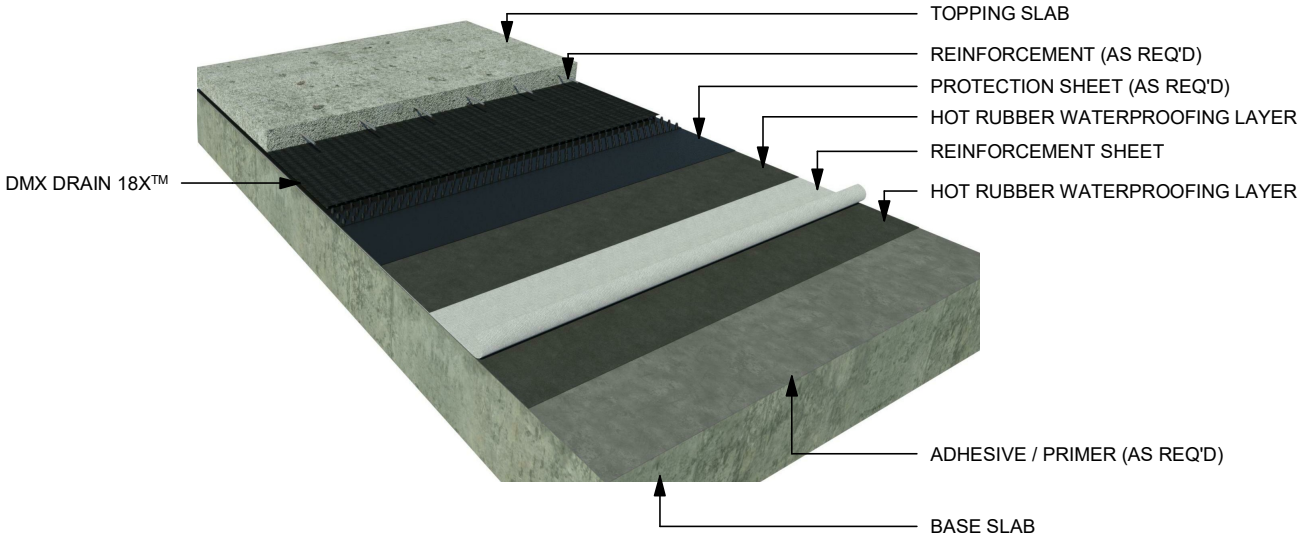
SPLIT SLAB WITH DMX DRAIN 18X™ (ISO)
