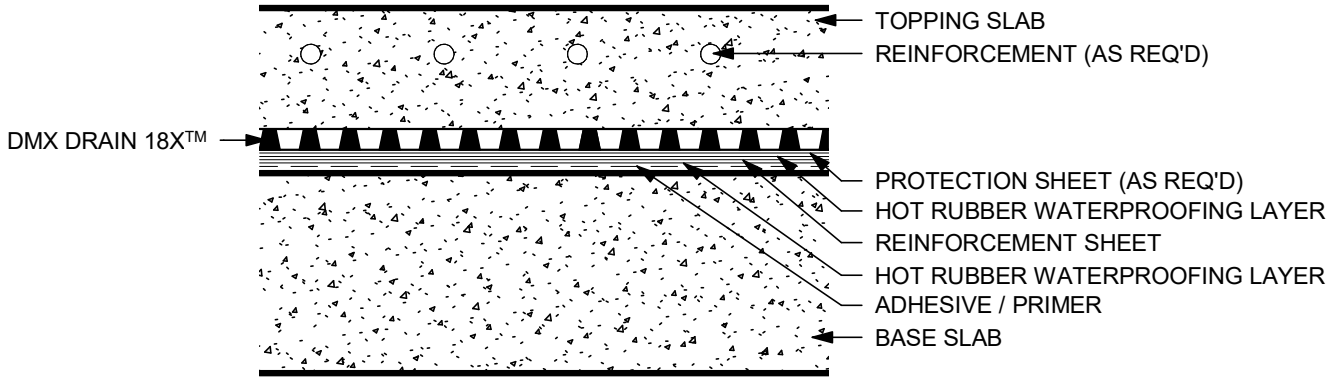
SPLIT SLAB WITH DMX DRAIN 18X™ (SECTION VIEW - N.T.S)
