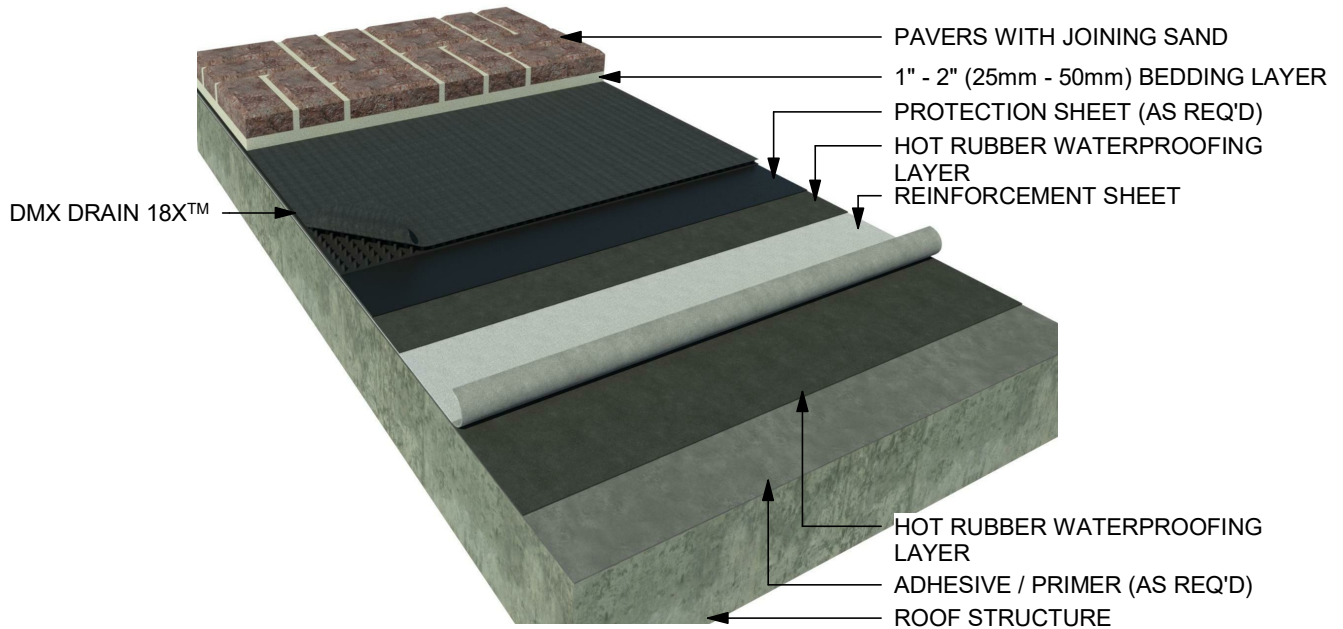
PAVERS ON DMX DRAIN 18X™ (ISO)
