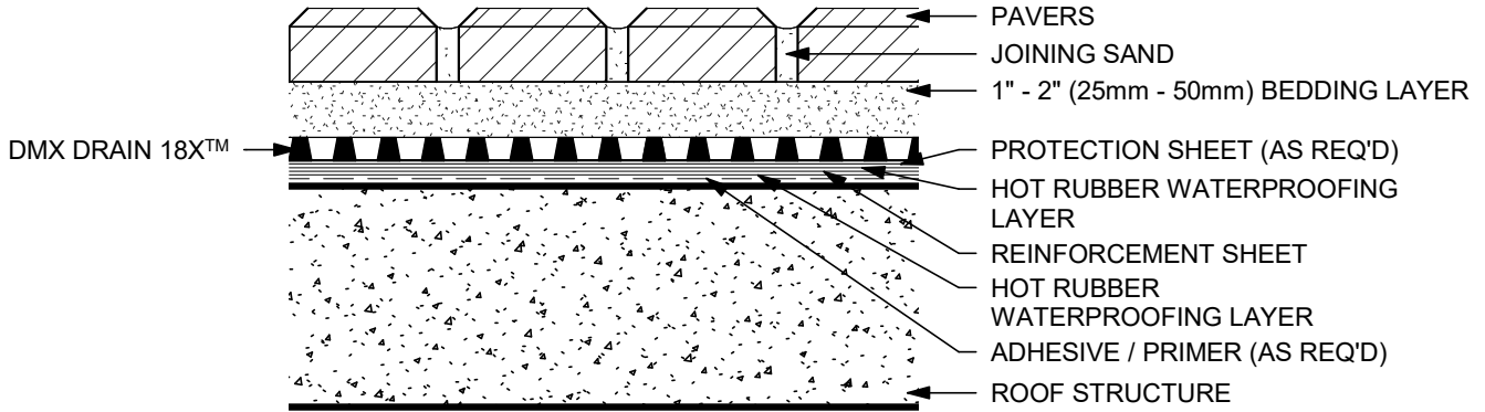
PAVERS ON DMX DRAIN 18X™ (SECTION VIEW - N.T.S)
