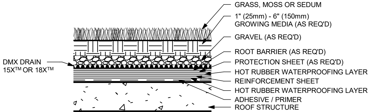
EXTENSIVE GREEN ROOF ON DMX DRAIN (SECTION VIEW - N.T.S)
