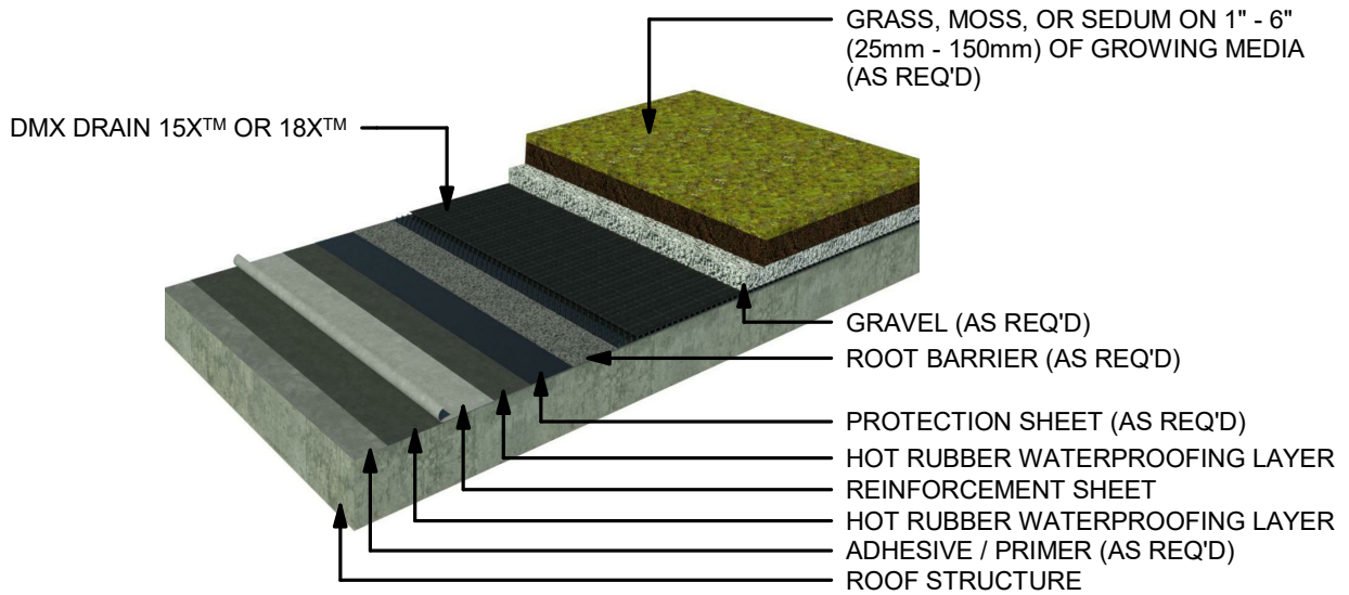
EXTENSIVE GREEN ROOF ON DMX DRAIN (ISO)
