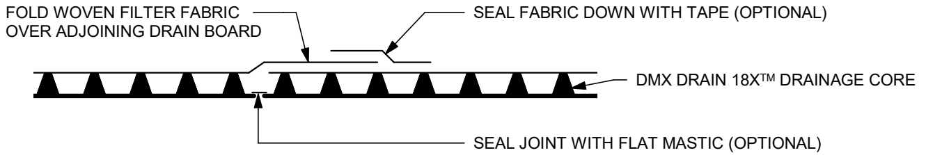
DMX DRAIN 18X™ HORIZONTAL OVERLAP (SECTION VIEW - N.T.S)
