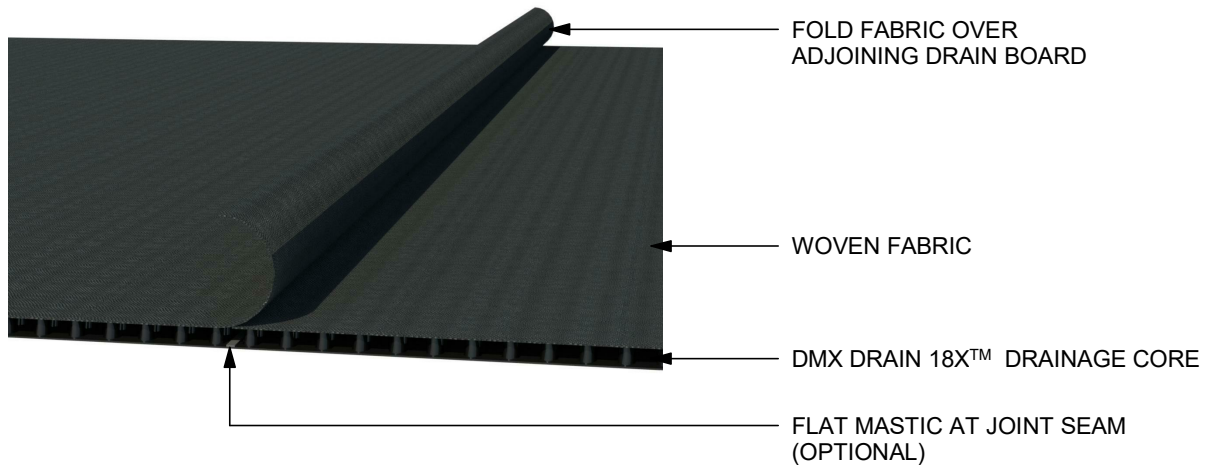
DMX DRAIN 18X™ HORIZONTAL OVERLAP (ISO)
