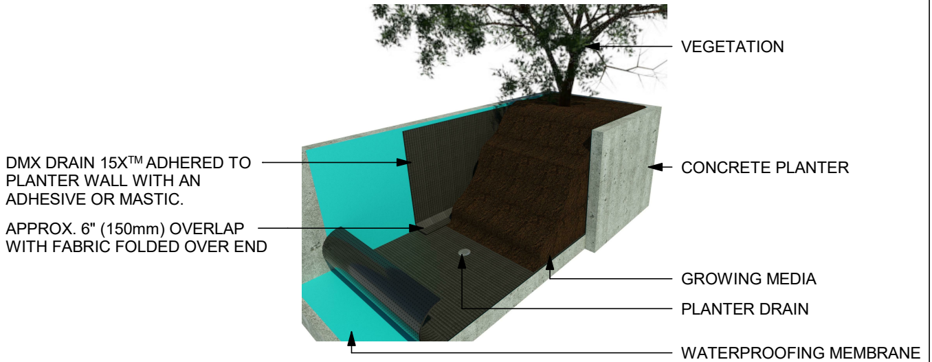
DMX 15X™ APPLIED TO PLANTER (ISO)
