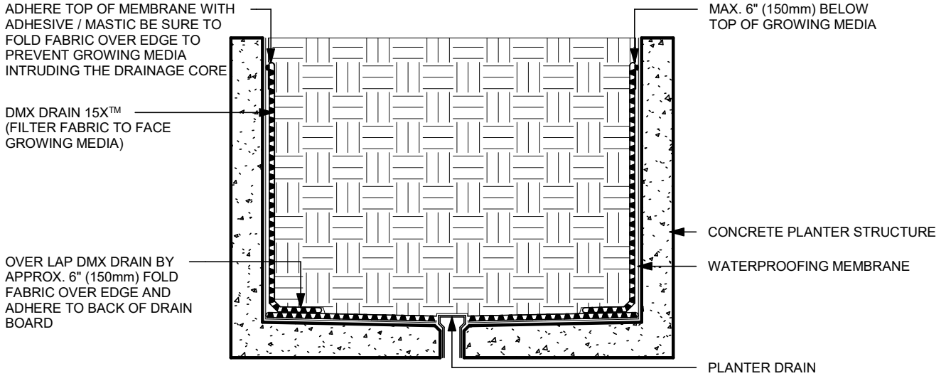
DMX DRAIN 15X™ APPLIED TO PLANTER (SECTION VIEW - N.T.S)
