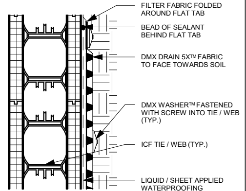
DMX DRAIN 5X™ ON ICF (SECTION VIEW - N.T.S)
