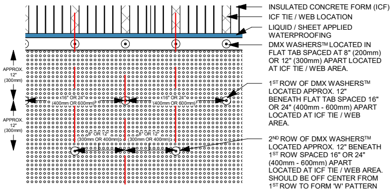
DMX DRAIN 5X™ ON ICF (FRONT VIEW - 1:20)
