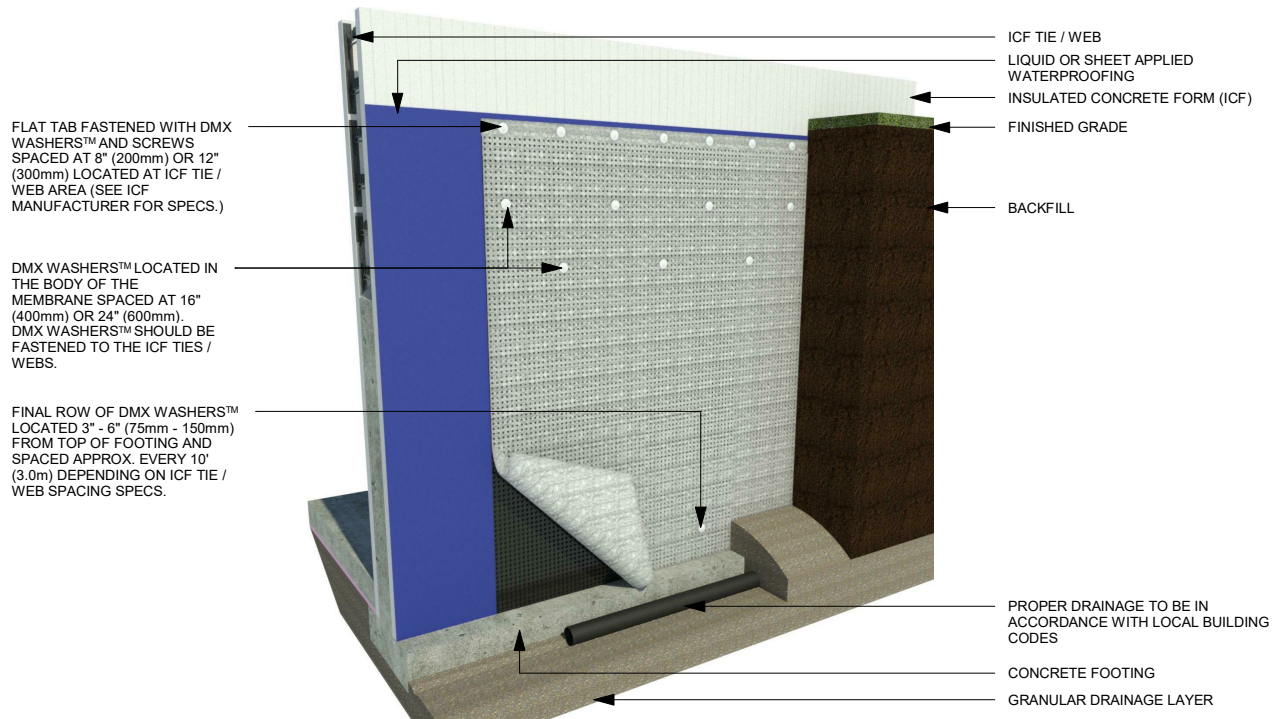
DMX DRAIN 5X™ ON ICF (ISO)
