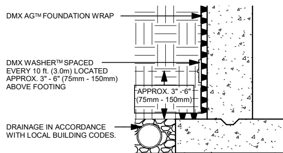
DMX AG™ AT FOOTING (SECTION VIEW - N.T.S)
