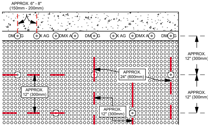
DMX AG™ ON CONCRETE FOUNDATION (FRONT VIEW - N.T.S)
