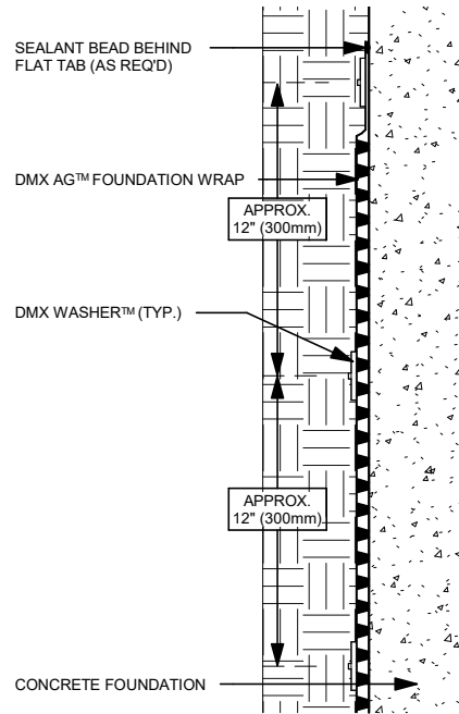
DMX AG™ ON CONCRETE FOUNDATION (SECTION VIEW - N.T.S)
