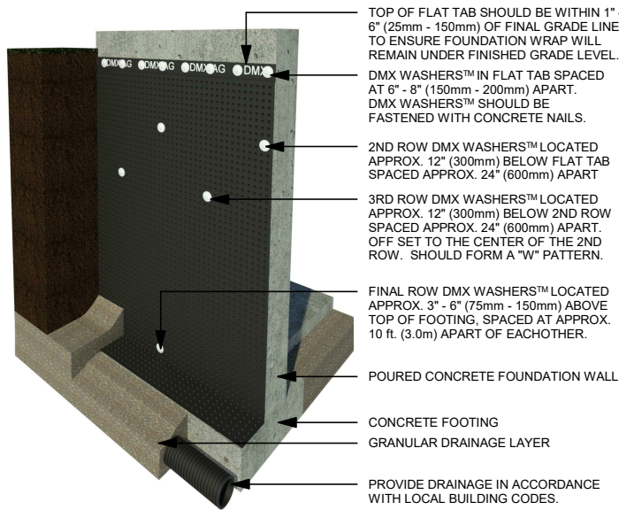
DMX AG™ ON CONCRETE W/ DMX WASHER™ PLACEMENT (ISO)
