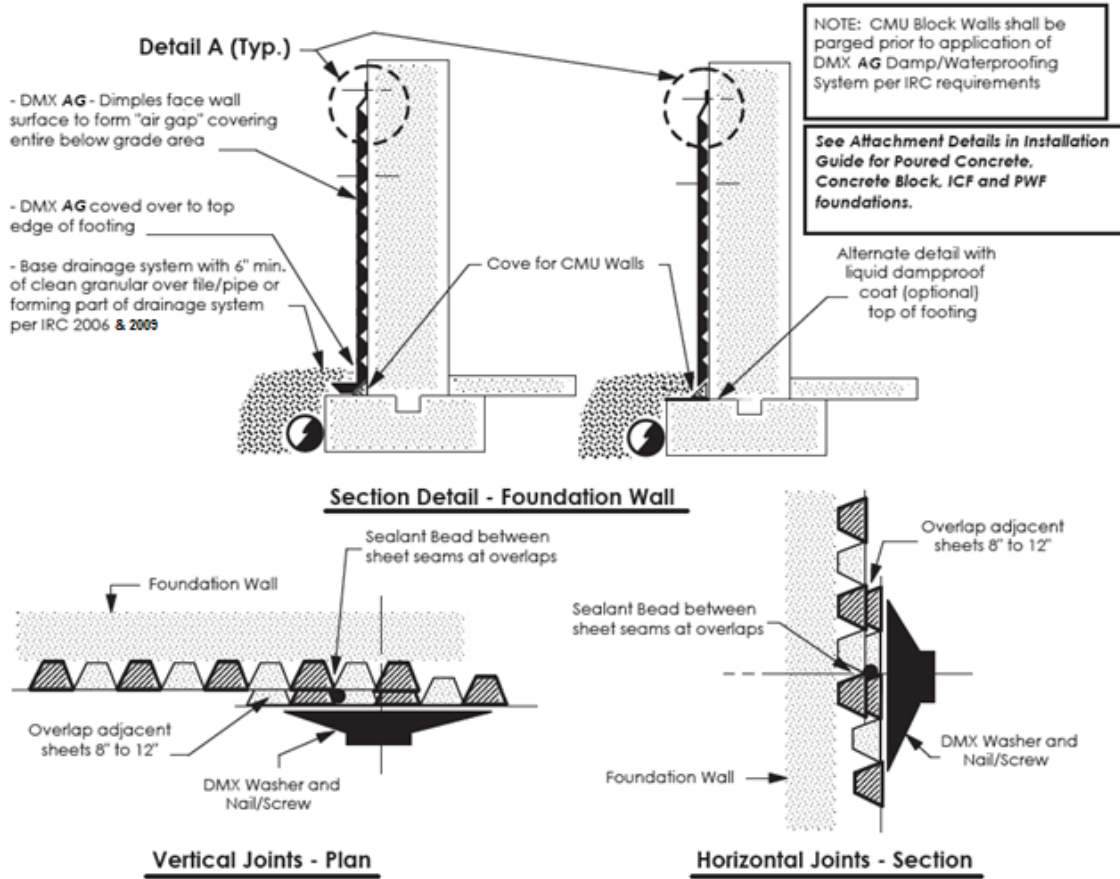
FIGURE 1—TYPICAL INSTALLATION DETAILS For SI: 1 inch = 25.4 mm
