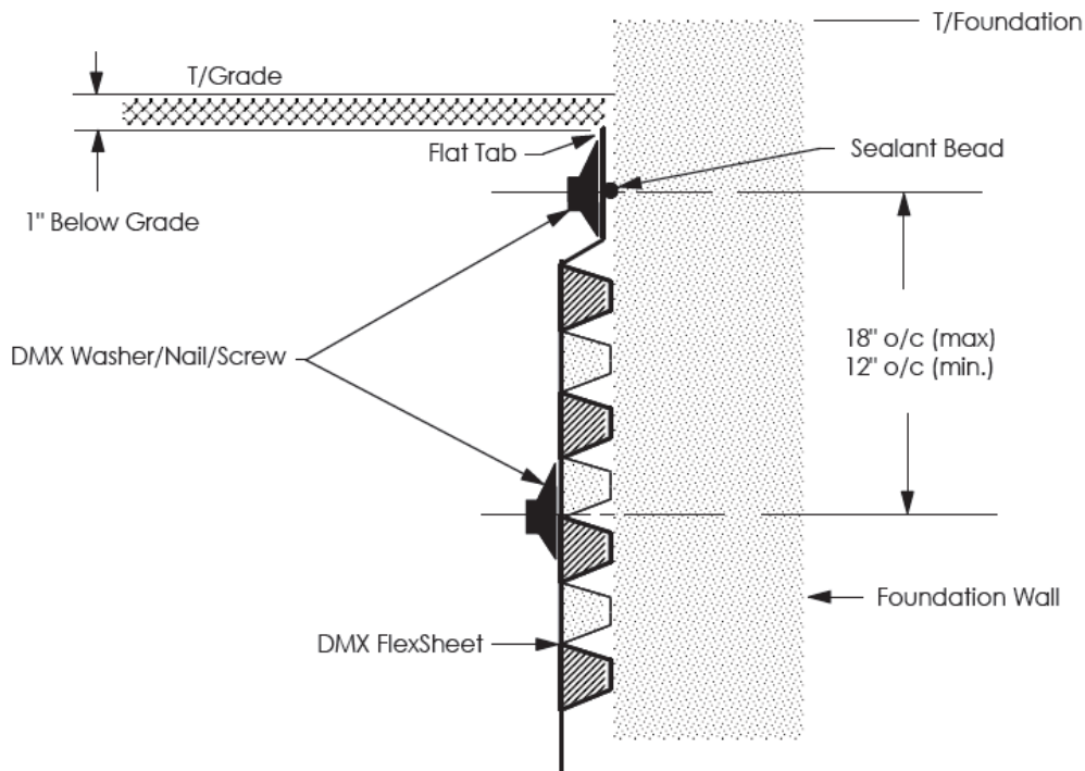
FIGURE 1—TYPICAL INSTALLATION DETAILS For SI: 1 inch = 25.4 mm
