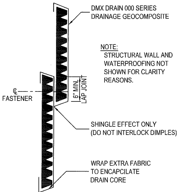
COMMERCIAL GRADE DRAINAGE BOARD HORIZONTAL LAP JOINTS (TYP.) VERTICAL APPLICATION
