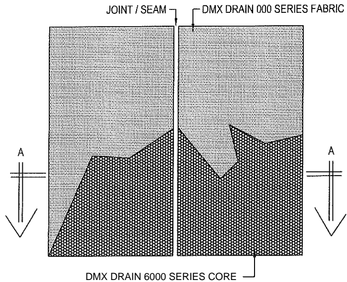
COMMERCIAL GRADE DRAINAGE BOARD SEALED BUTT JOINTS (TYP.) HORIZONTAL APPLICATION
