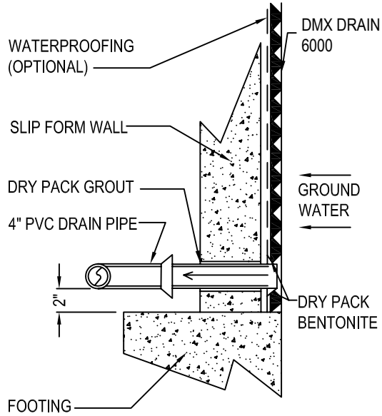
DETAIL 'B'
