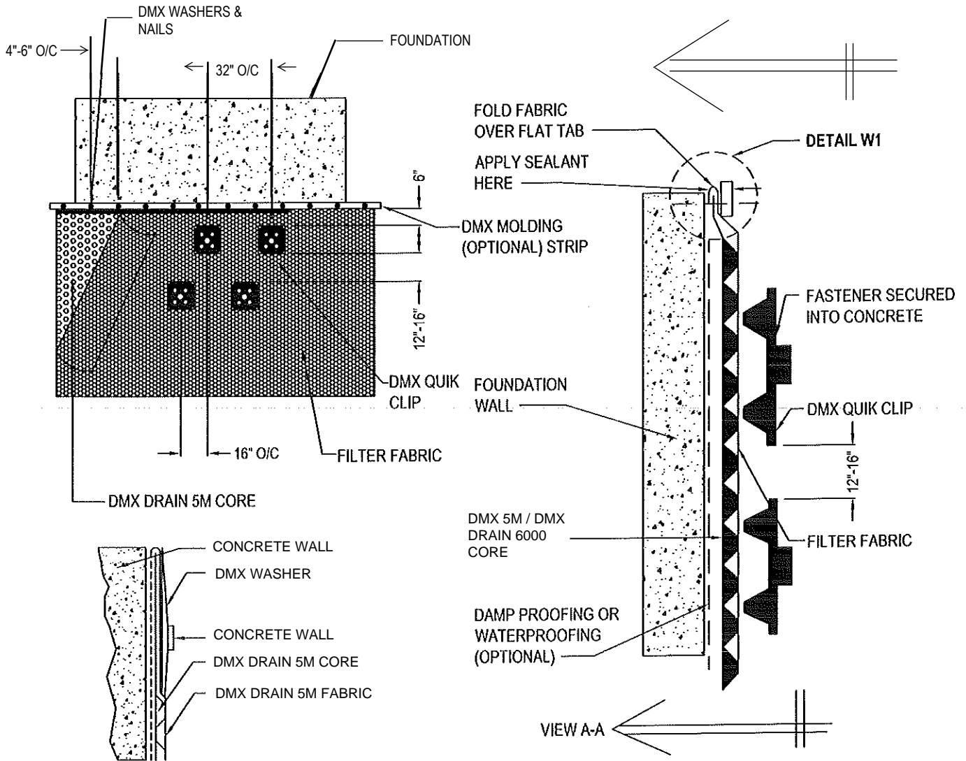
DETAIL W1
