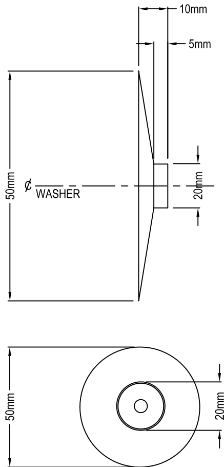
DMX WASHER DIMENSIONS FOR DMX AG
